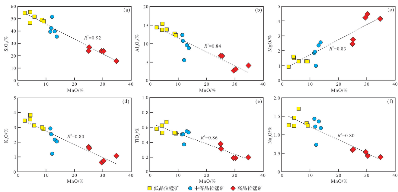
图2 民乐地区大塘坡组不同品位锰矿主量元素特征 Fig.2 Major element vs. MnO content in manganese ores from the Datangpo Formation, Minle area
